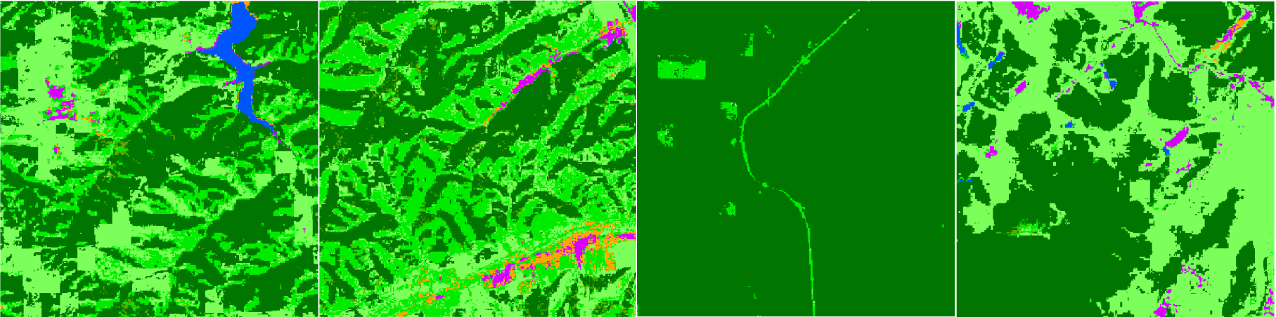
(b) FROM-GLC
